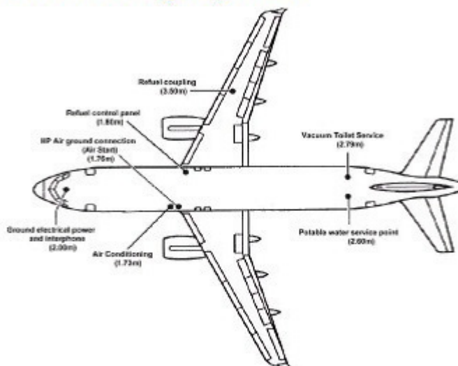
A319/320/321 Servicing Connection Locations (height above ground in metres)
