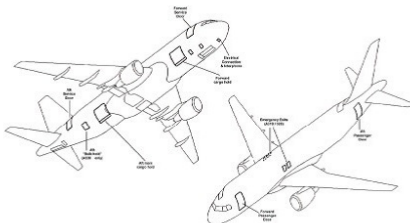
Main forward and aft cargo compartments.
