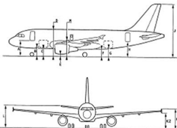
Ground Clearances/Sill Heights (metres. Nominal values. Allow \pm 0.076 m)
