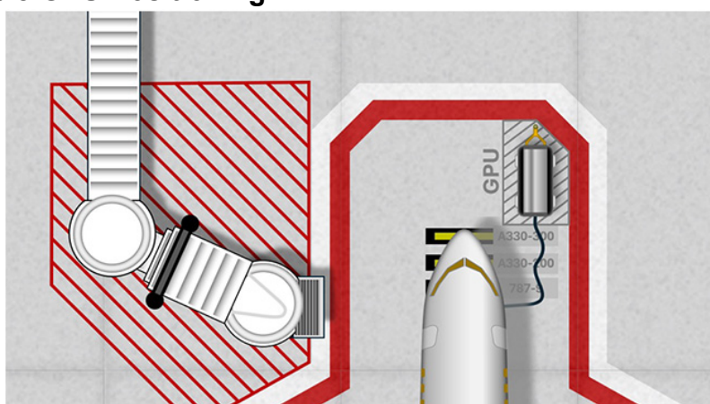
Figure 4.8 Sample GPU Positioning
