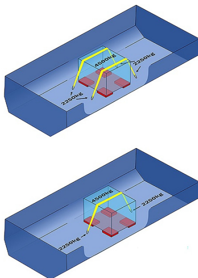
Figure 4.9 Examples of Embraced Load Lashing
