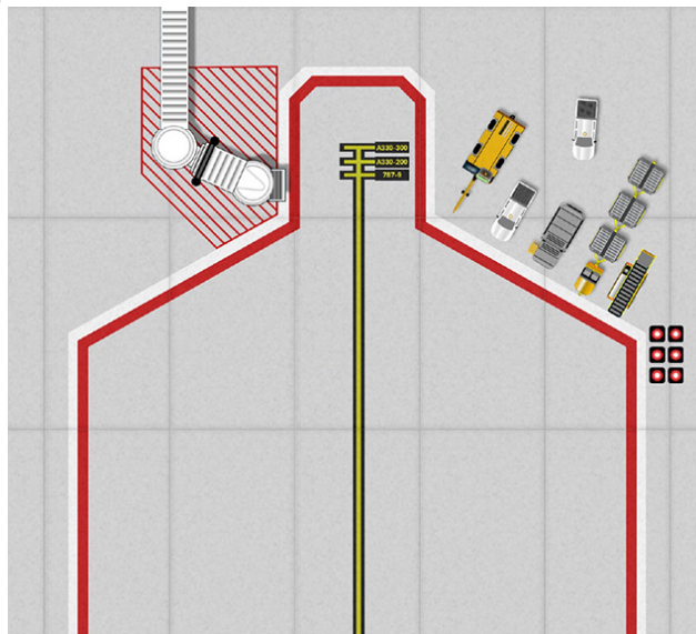
Figure 4.7 During aircraft pre-arrival, all personnel and equipment must position well clear of the aircraft's path
