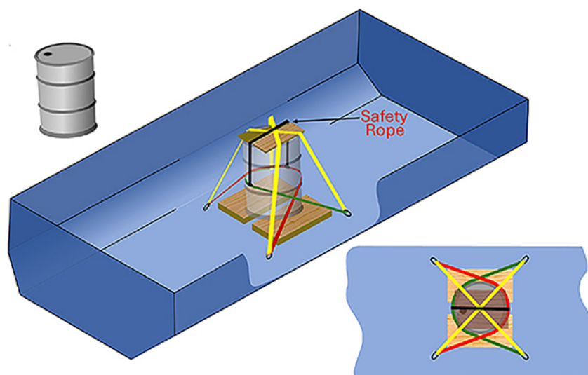
Figure 4.18 Lash Barrels with Protective Planks
