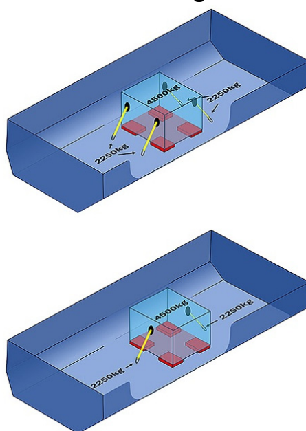
Figure 4.10 Examples of Direct Load Lashing
