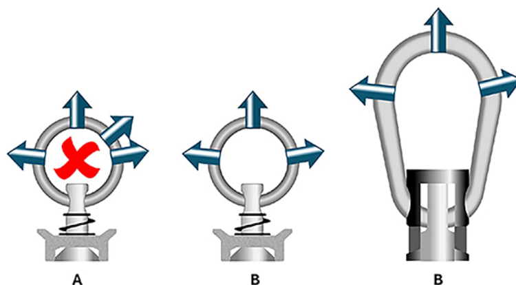
Figure 4.11 Tie-down Fitting with Maximum Three Straps/Ropes in Three Different Restraint Directions
