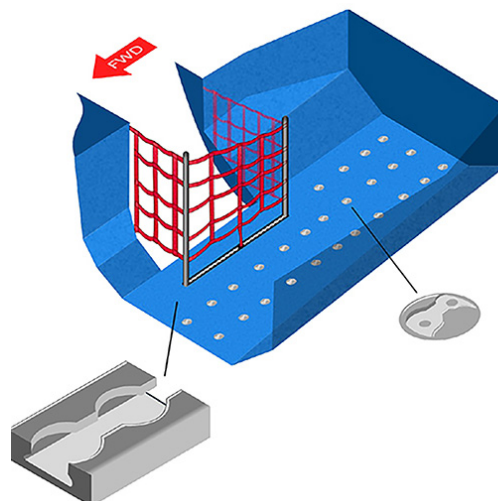
Figure 4.14 Example of Tie-down Attachment Points in the Bulk Compartment
