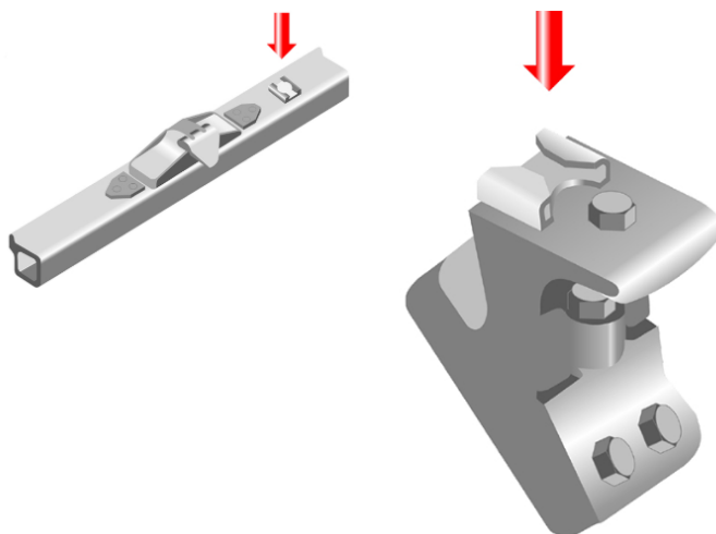
Figure 4.12 Example of Tie-down Attachment Points on Outboard Side Lock and Side Guide
