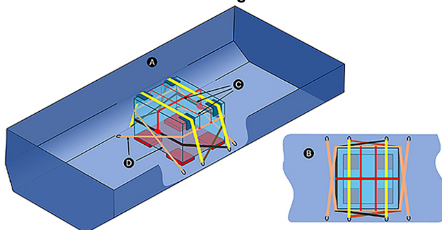
Figure 4.17 Standard and Sideward Lashing of a Load
