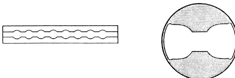
Figure 4.4 Example of Tie-down Attachment Points on Track and Anchor Plate
