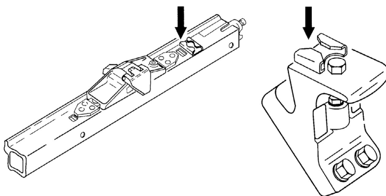
Figure 4.3 Example of Tie-down Attachment Points on Outboard Side Lock and Side Guide
