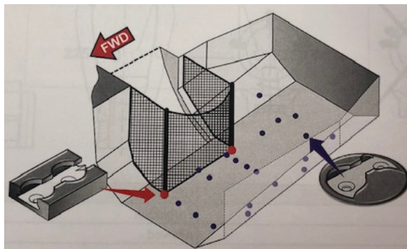
Figure 4.5 Example of Tie-down Attachment Points in the Bulk Compartment
