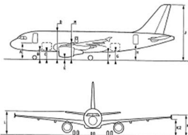
Ground Clearances/Sill Heights (metres. Nominal values. Allow \pm 0.076 m)
