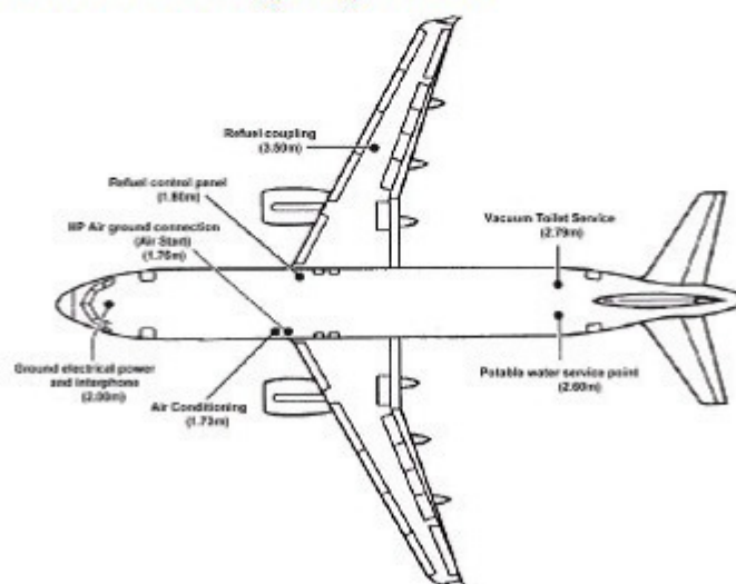
A319/320/321 Servicing Connection Locations (height above ground in metres)
