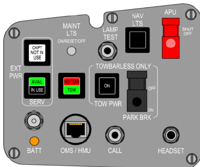
ELECTRICAL/TOWING SERVICE PANEL
